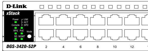
Figure 1- 12. LED indicators for the DGS-3420-52P
