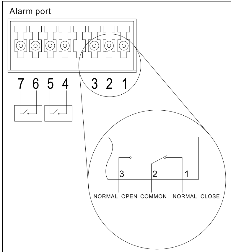
Figure 2-4 Alarm Connector
